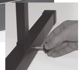
1" Finger bolt is threaded into upright from outside of base bar
